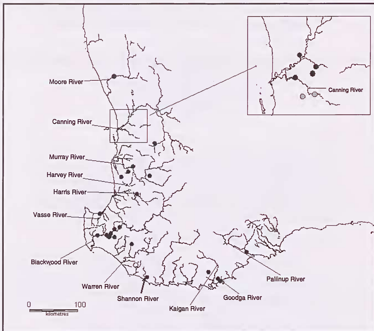
Figure 1. Southwest Coast Drainage Division, showing sampling locations. Black circles indicate that no fishes from that location were infested with Lernaea , grey circles indicate that Lernaea were found on some sampled fishes.
